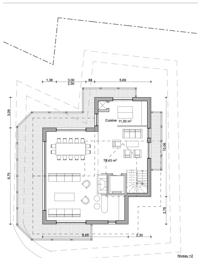
ETAGE 2 / FLOOR 2
